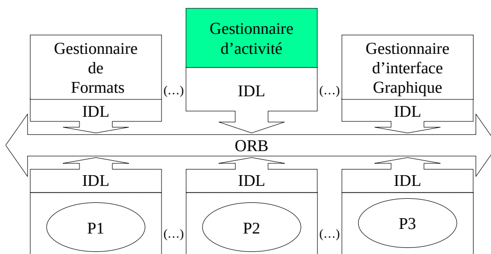
Figure 3.5 – Architecture d'EduMed
